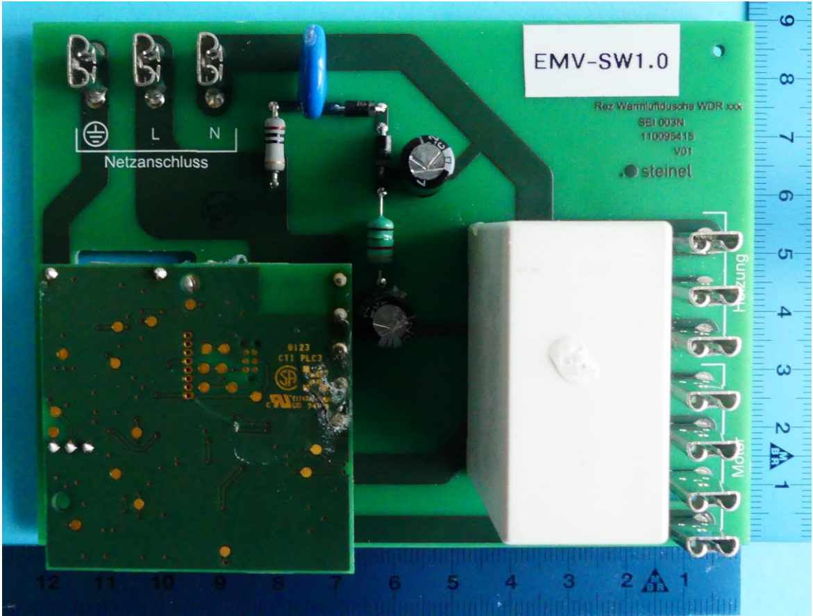
PCB, top side view
